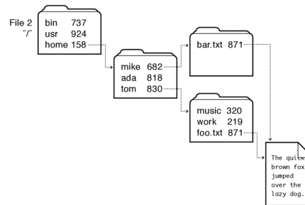
Figure 1: Hard link
